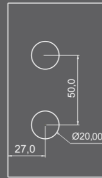
HE 1114 / HE 1115
