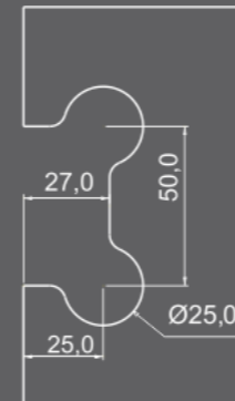
HE 1310
